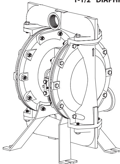
ALUMINUM PUMP
